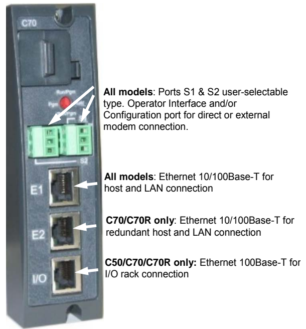
Figure 1 Communication ports
