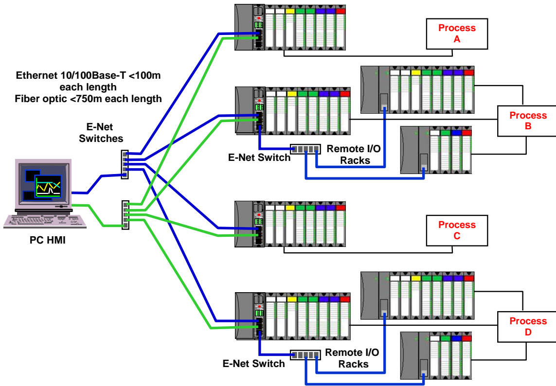
Multiple processes/multiple racks/C70 controller redundant networks
