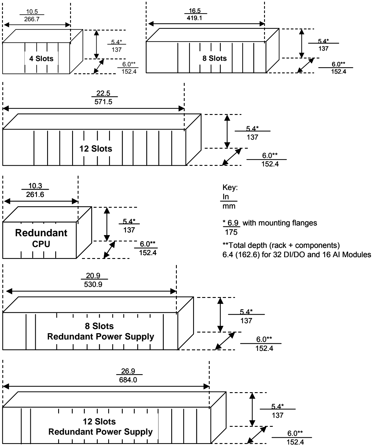
Figure 2 HC900 Hybrid Controller Dimensions
