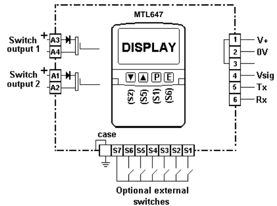
Fig 1 Simplified block diagram of MTL647
