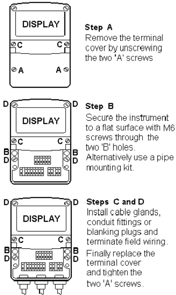
Fig 6 MTL647 installation procedure
